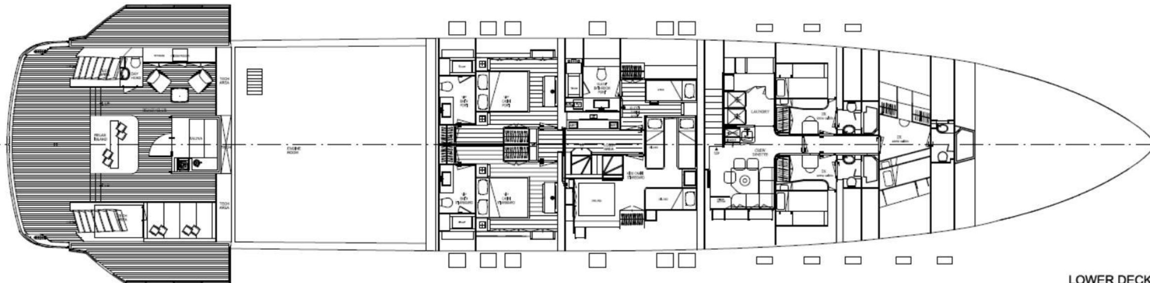
LOWER DECK
